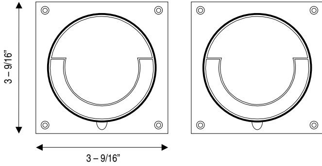
REVOLVING RING FLUSH HANDLES ~ S1952 ## 1001
