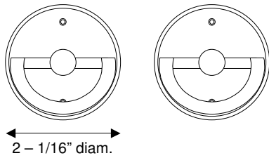
ROUND FLUSH LATCH HANDLE ~ S1954 ## 1001
