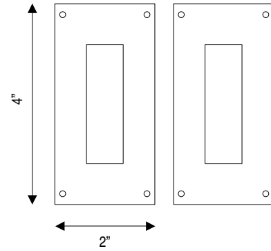
PLAIN FLUSH PULL ~ S1405 ## 1001
