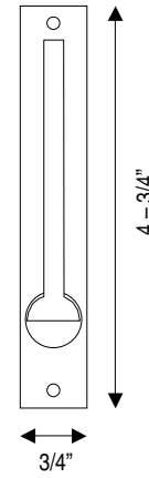
PLAIN FLUSH PULL ~ S1405 ## 1001
